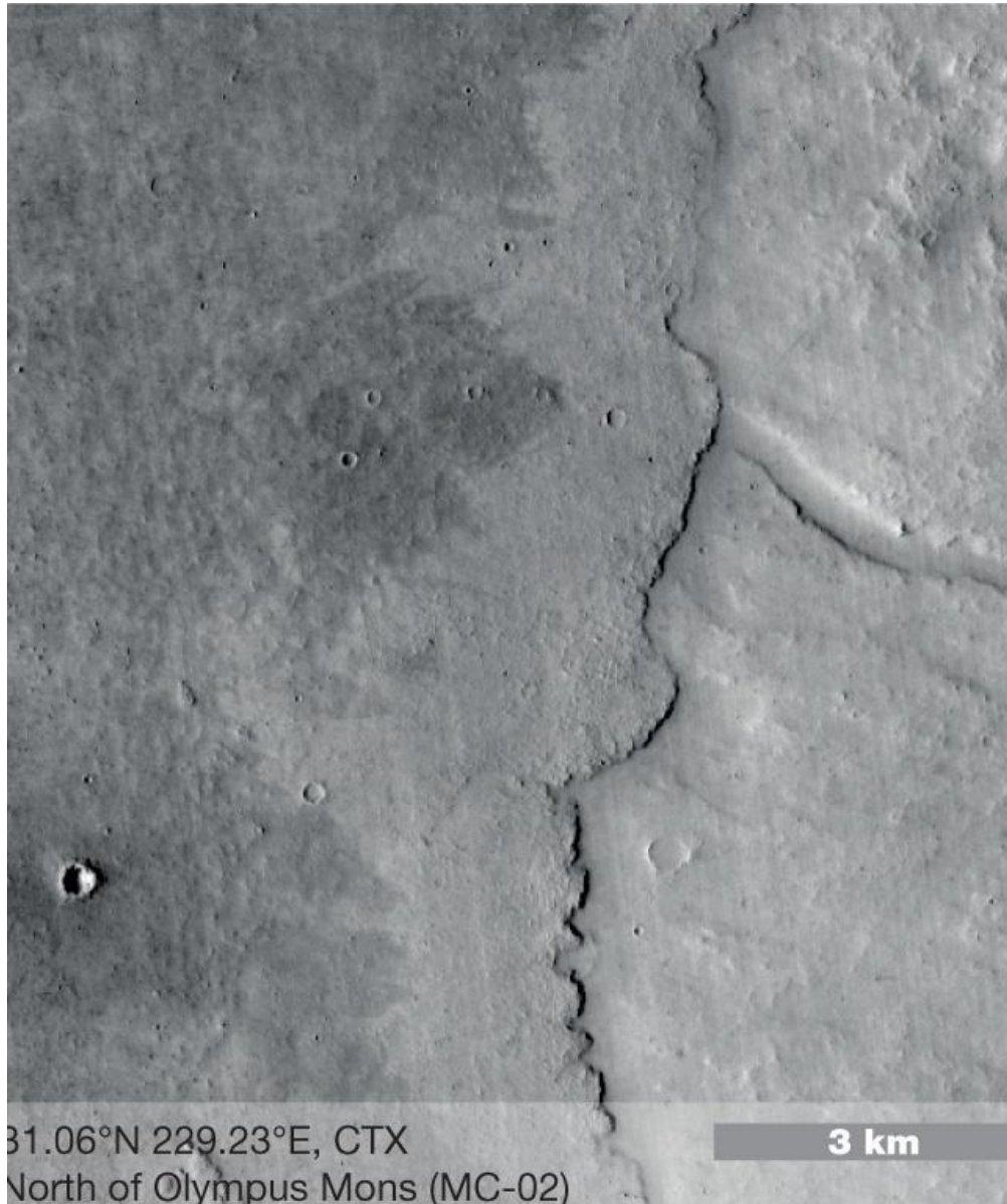
IMAGE 2: North of Olympus Mons, Mars.
