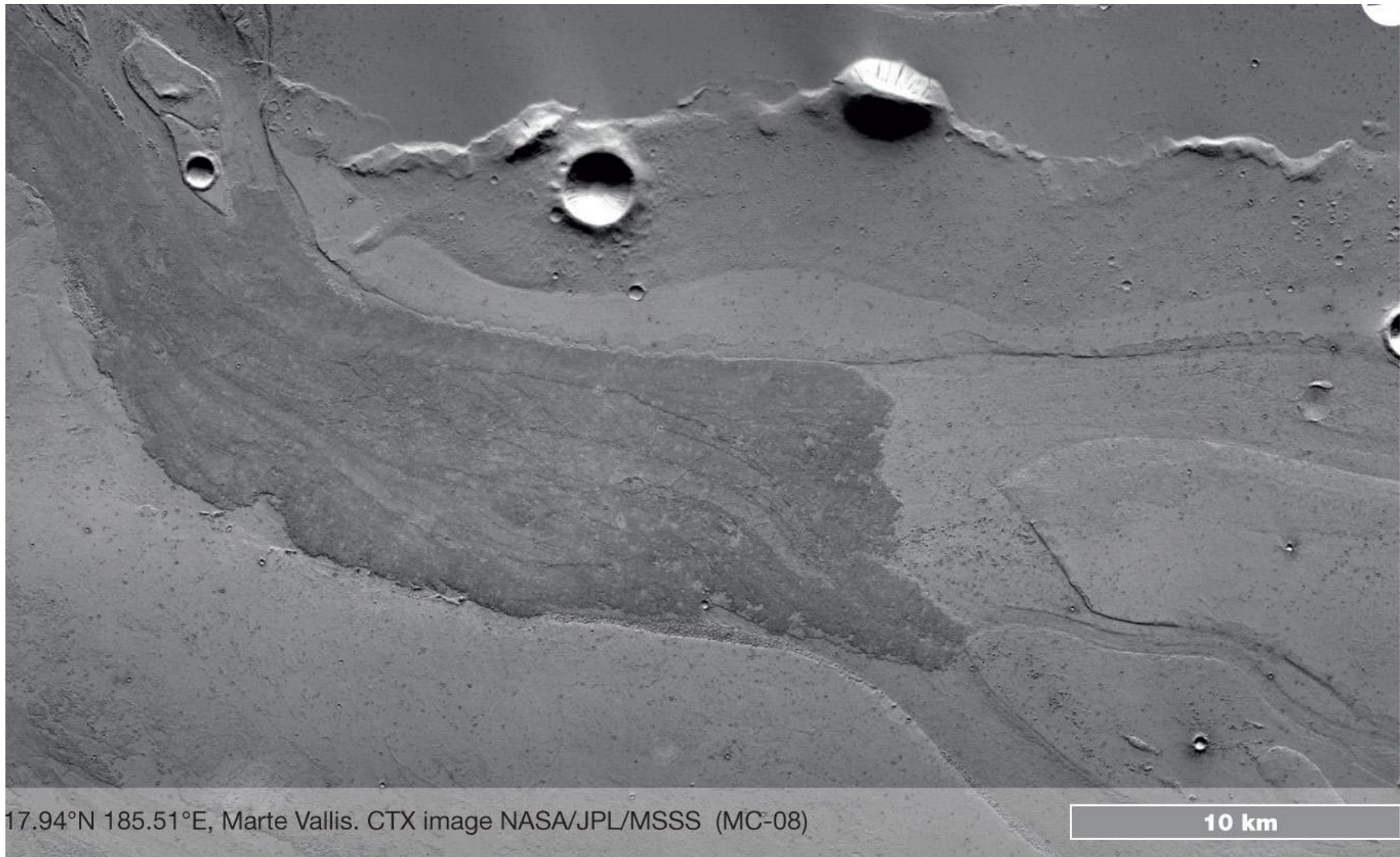
IMAGE 1: Marte Vallis, Mars, East of Elysium Mons.
